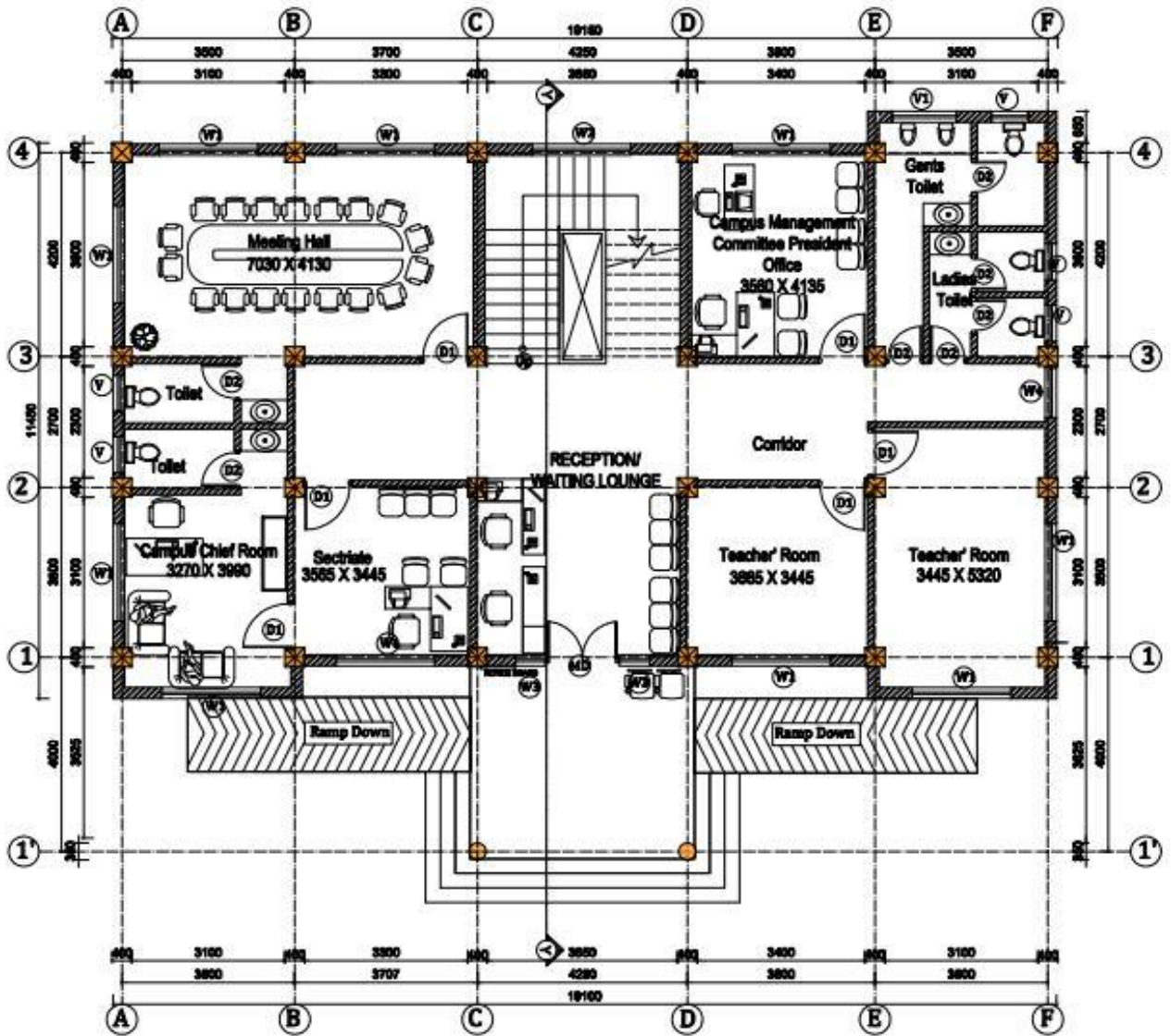
Ground Floor Plan Area = (235.87 Sq.m)
